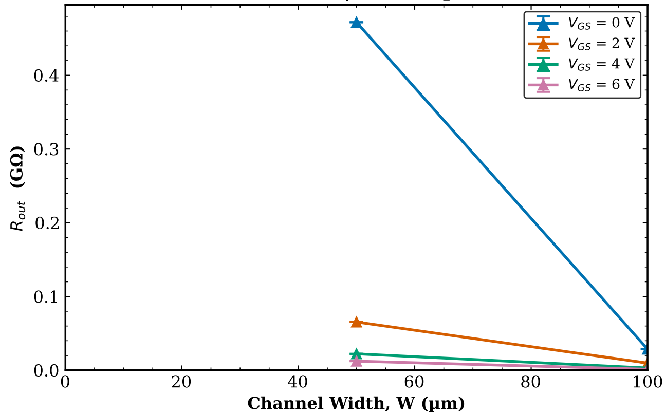
TFT3 Transistor 1 R_{out} vs W | L = 40\text{ }\mu\text{m}
